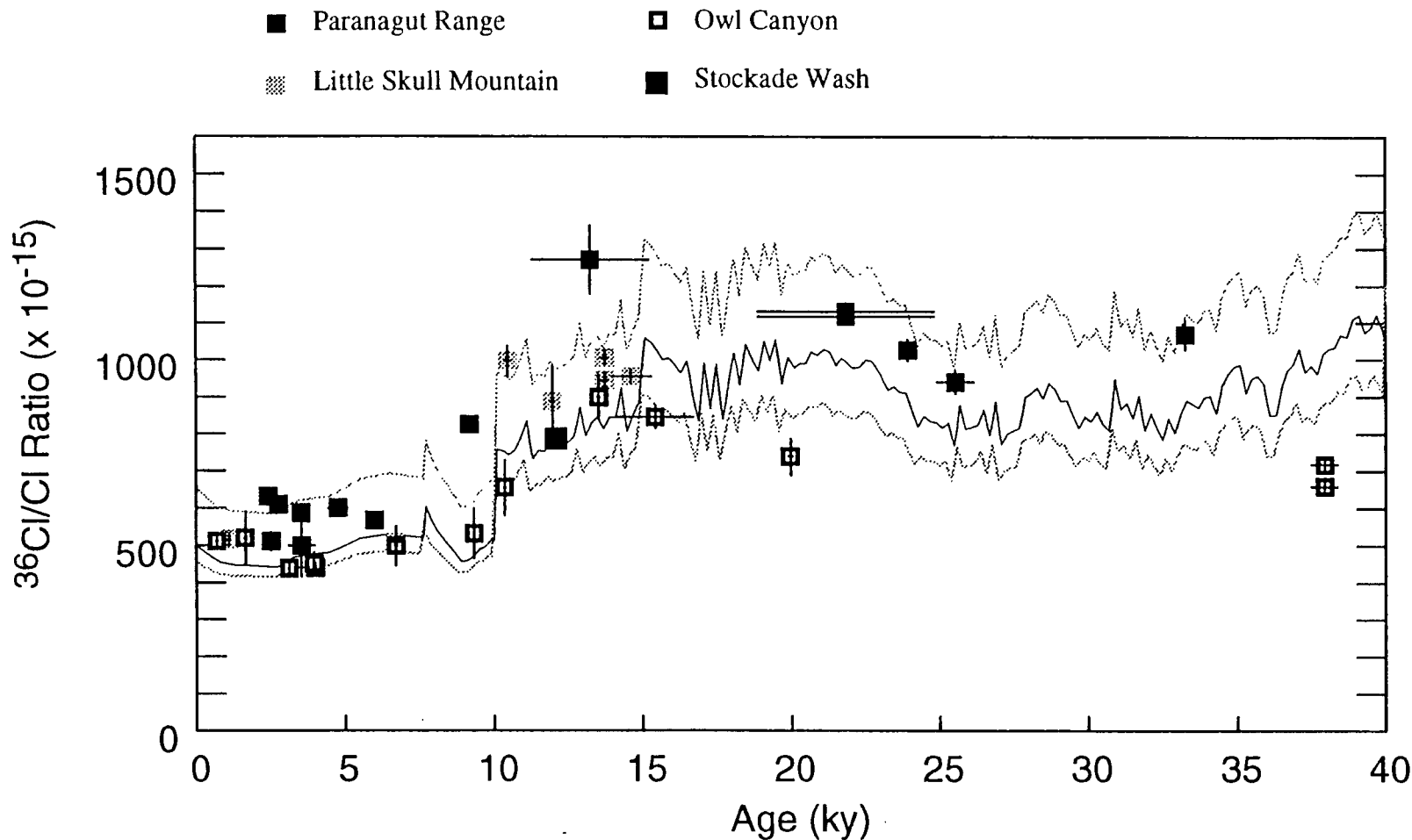
Figure 2-2. Reconstructed production rate of chlorine-36 in the atmosphere, compared against measured data for packrat middens from the vicinity of the Nevada Test Site. The reconstructed ^{36}\text{Cl}/\text{Cl} ratio shown by the solid line assumes that the deposition rate of stable chloride was constant at present day rates during the Holocene (i.e., ages less than 10 ky) but 33% lower throughout the Pleistocene. Lower and upper limits shown by the gray lines assume present-day ^{36}\text{Cl}/\text{Cl} ratios of 450 \times 10^{-15} and 650 \times 10^{-15} , respectively. See section 2.1 for a discussion of these reconstructions.
